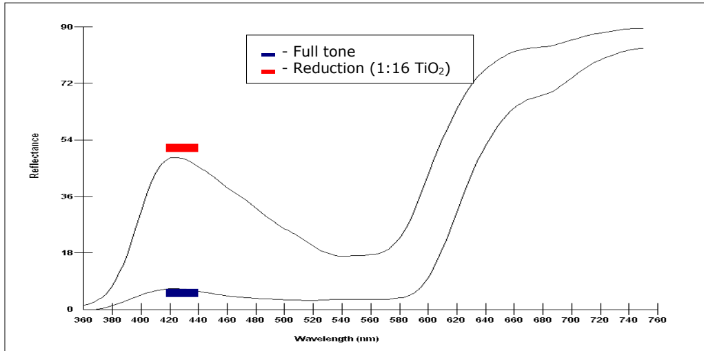
Full tone, Reduction [1:16 TiO 2 ] & [1:50 TiO 2 ] Reflectance Curve – Alkyd/melamine Paint Full Shade (5%) & Reduction (1:16 TiO 2 )
